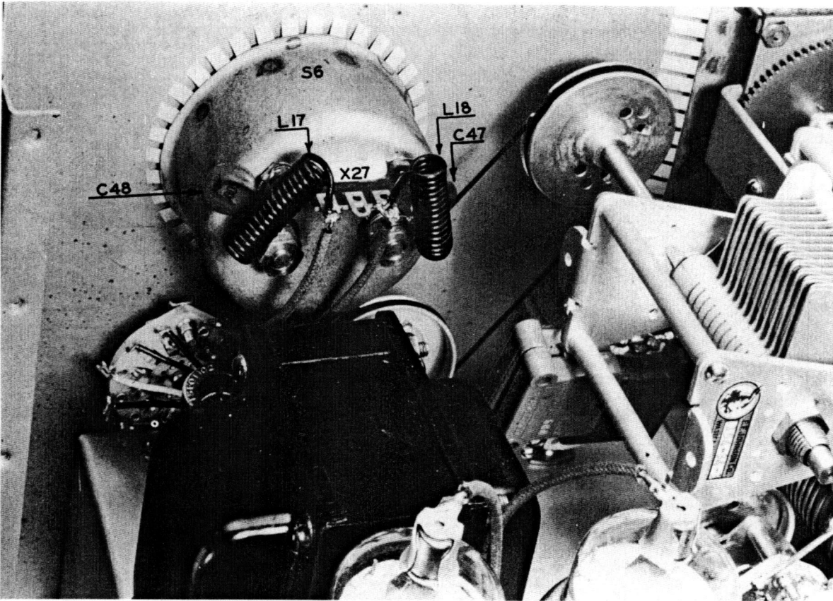
Figure 10a — Meter Filter Detail
