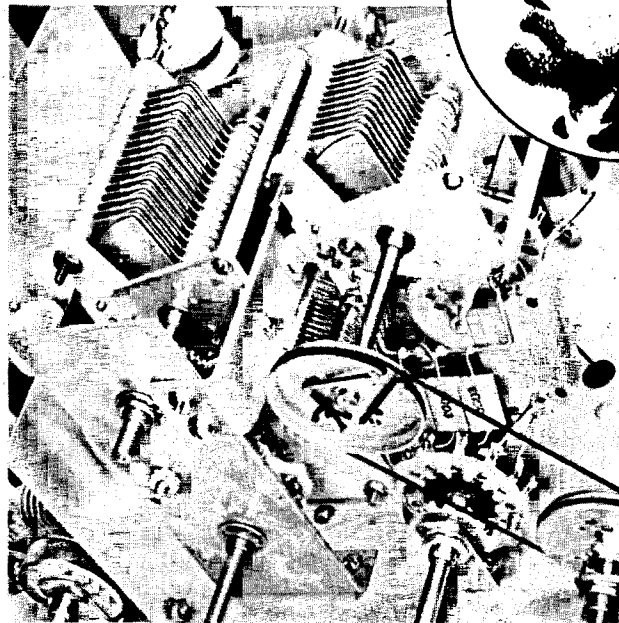
Figure 2. Pi-network Coupling System
