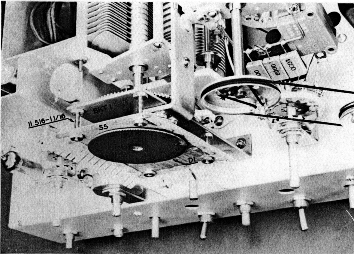
Figure 10b — Dial Window Shield Detail
