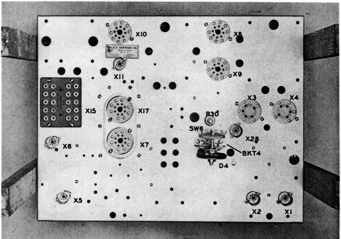
Figure 1 — Socket Mounting
