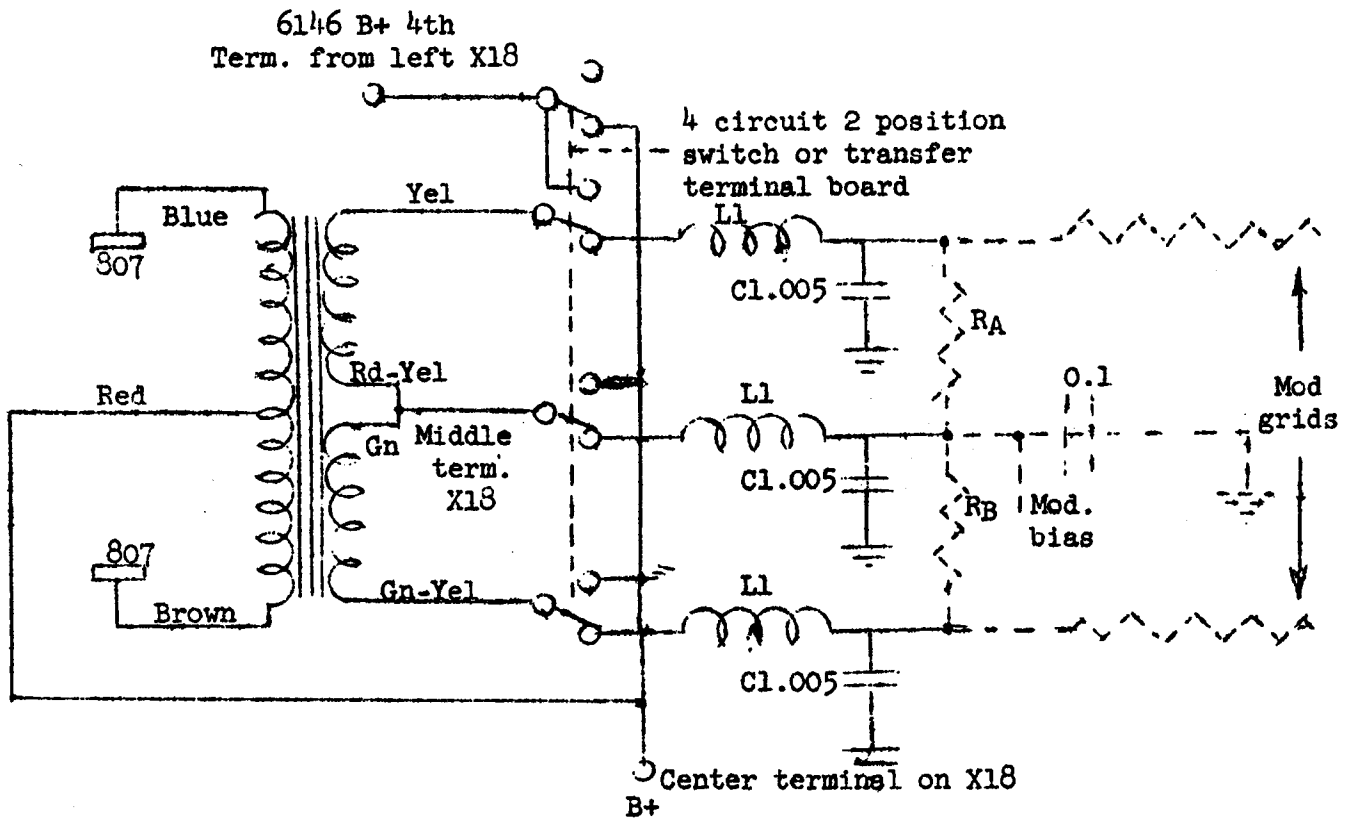
FIGURE A DIRECT GRID CONNECTION
