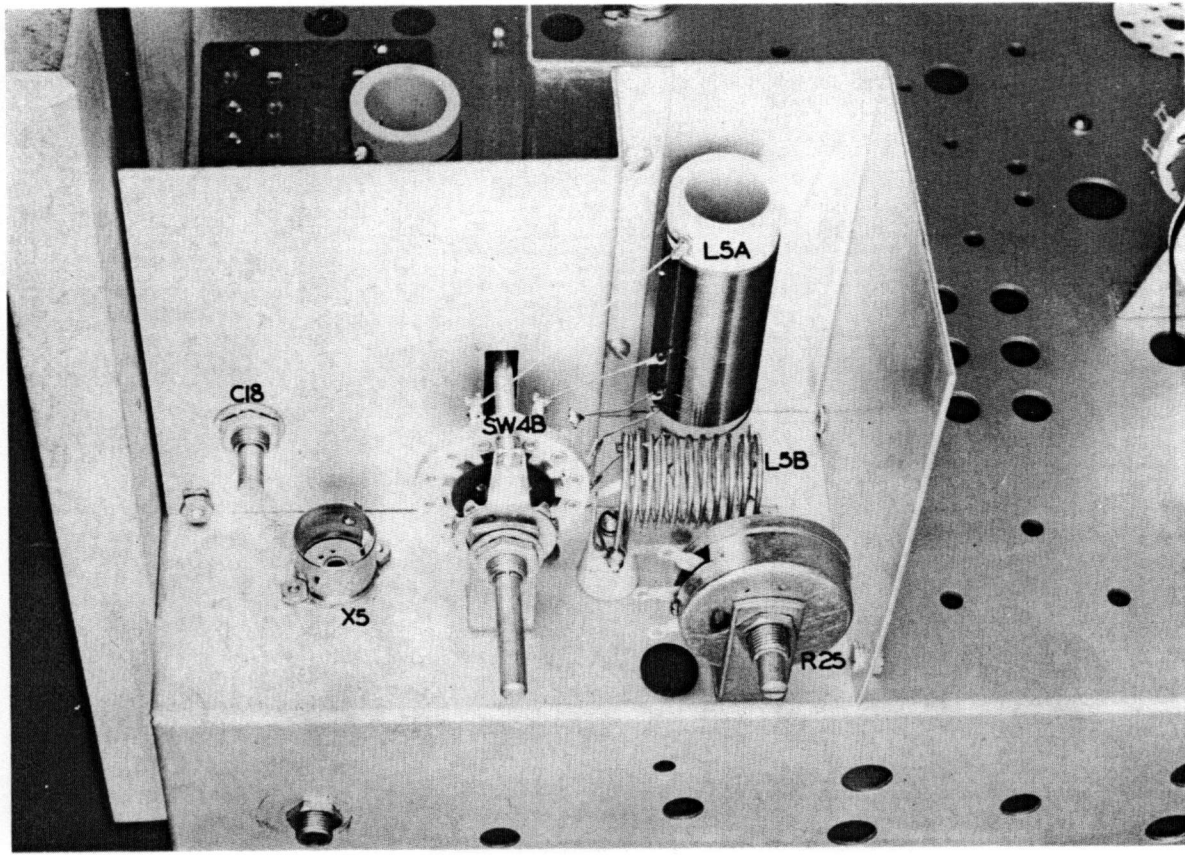
Figure 4 — Buffer Assembly Detail
