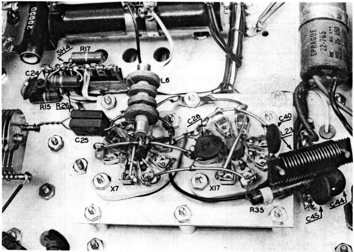
Figure 10c—6146 Socket Wiring
