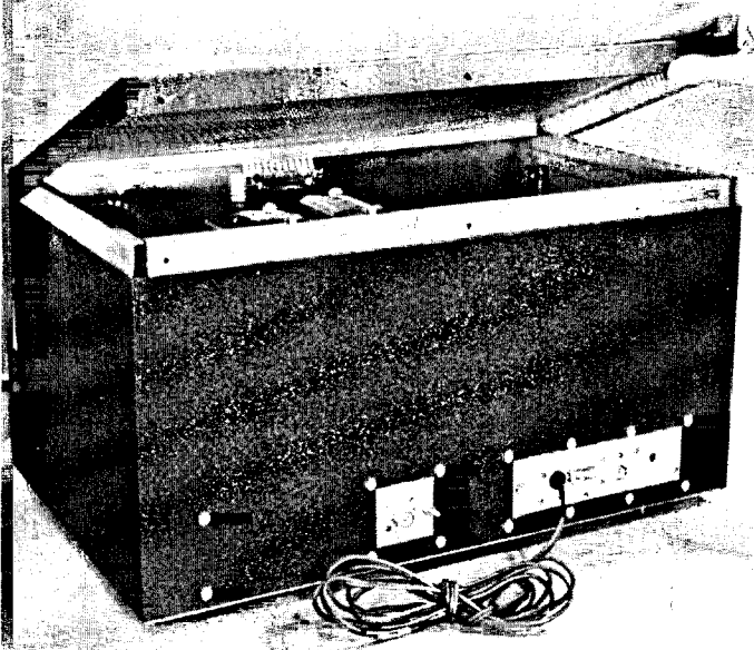
Figure 4. Lid Removal, Showing Phosphor Bronze Bonding Fingers
