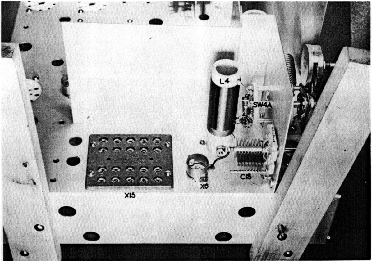
Figure 5 — Oscillator Assembly Detail
