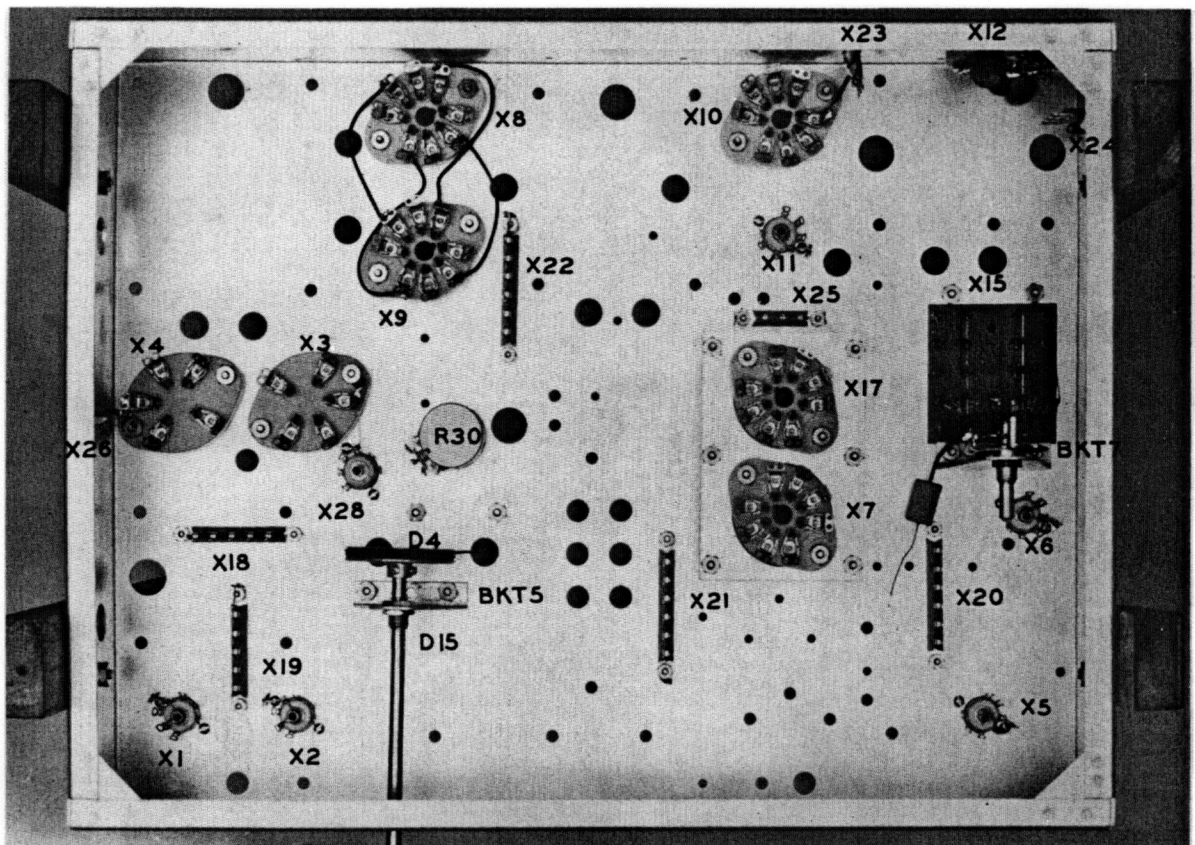
Figure 2 — Socket and Terminal Board Mounting
