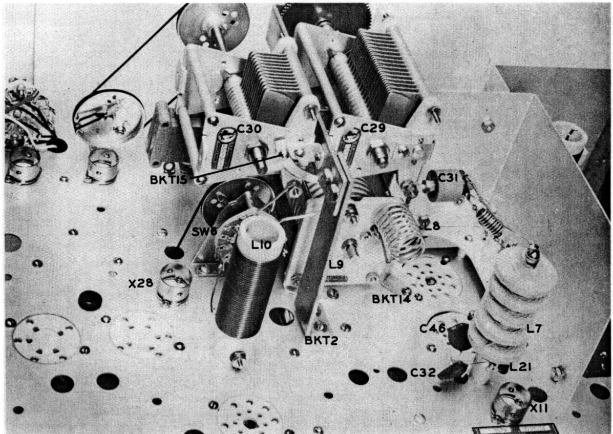
Figure 6-7 — PA Assembly Detail
