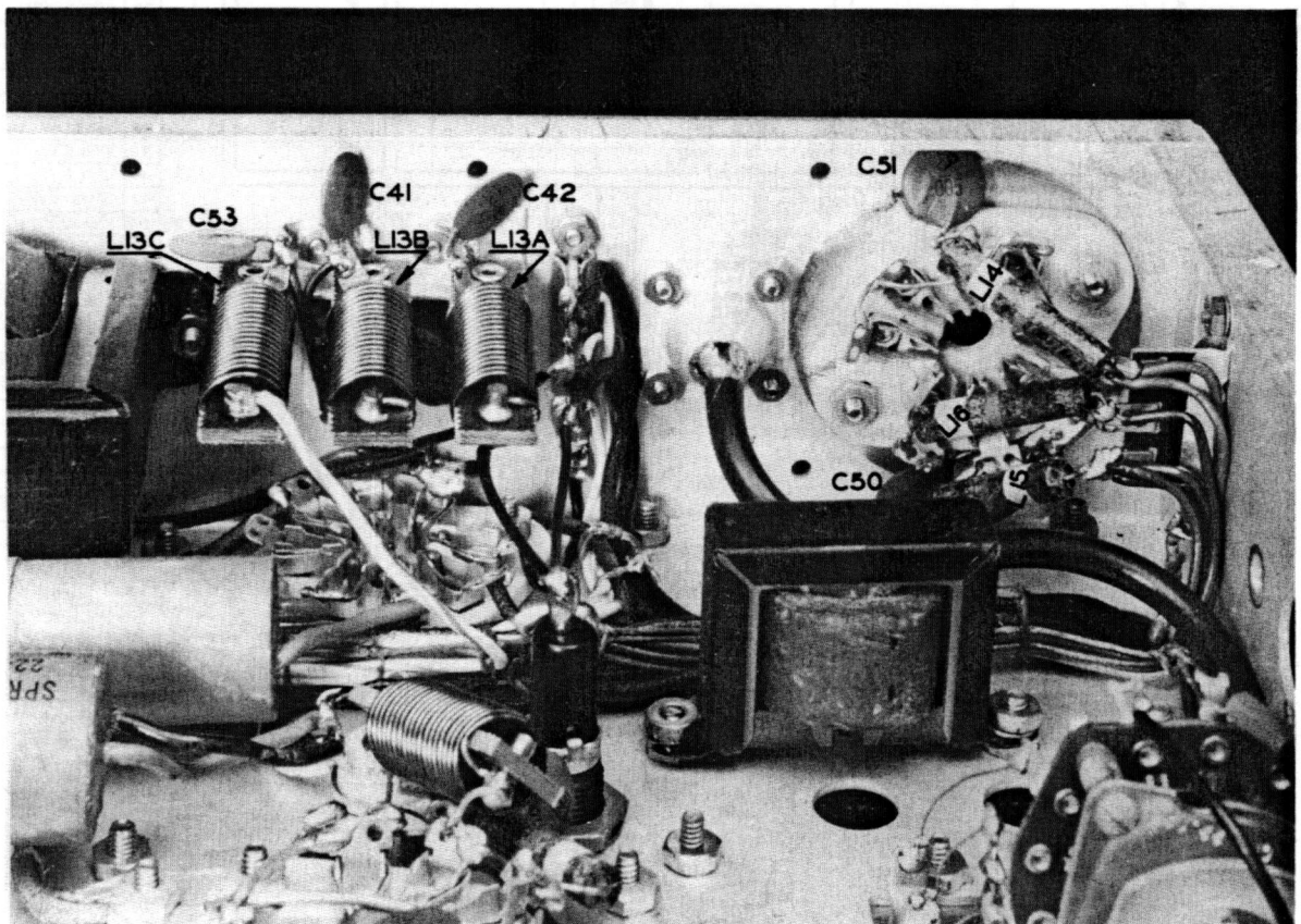
Figure 10d—Line Filter, VFO Socket Wiring Detail
