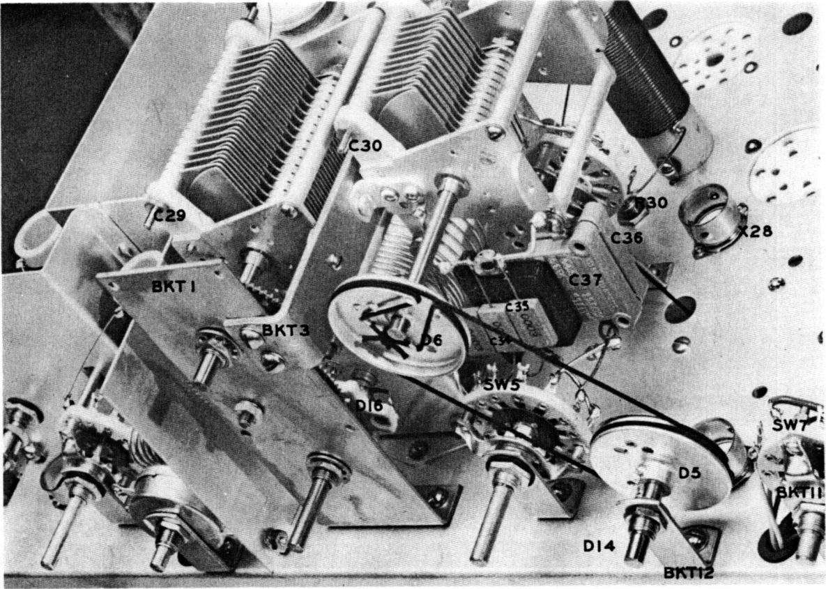
Figure 3 — PA Assembly Detail
