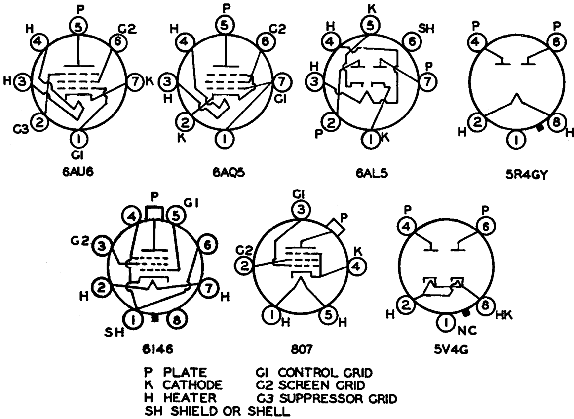
Figure 13—Socket Connections
